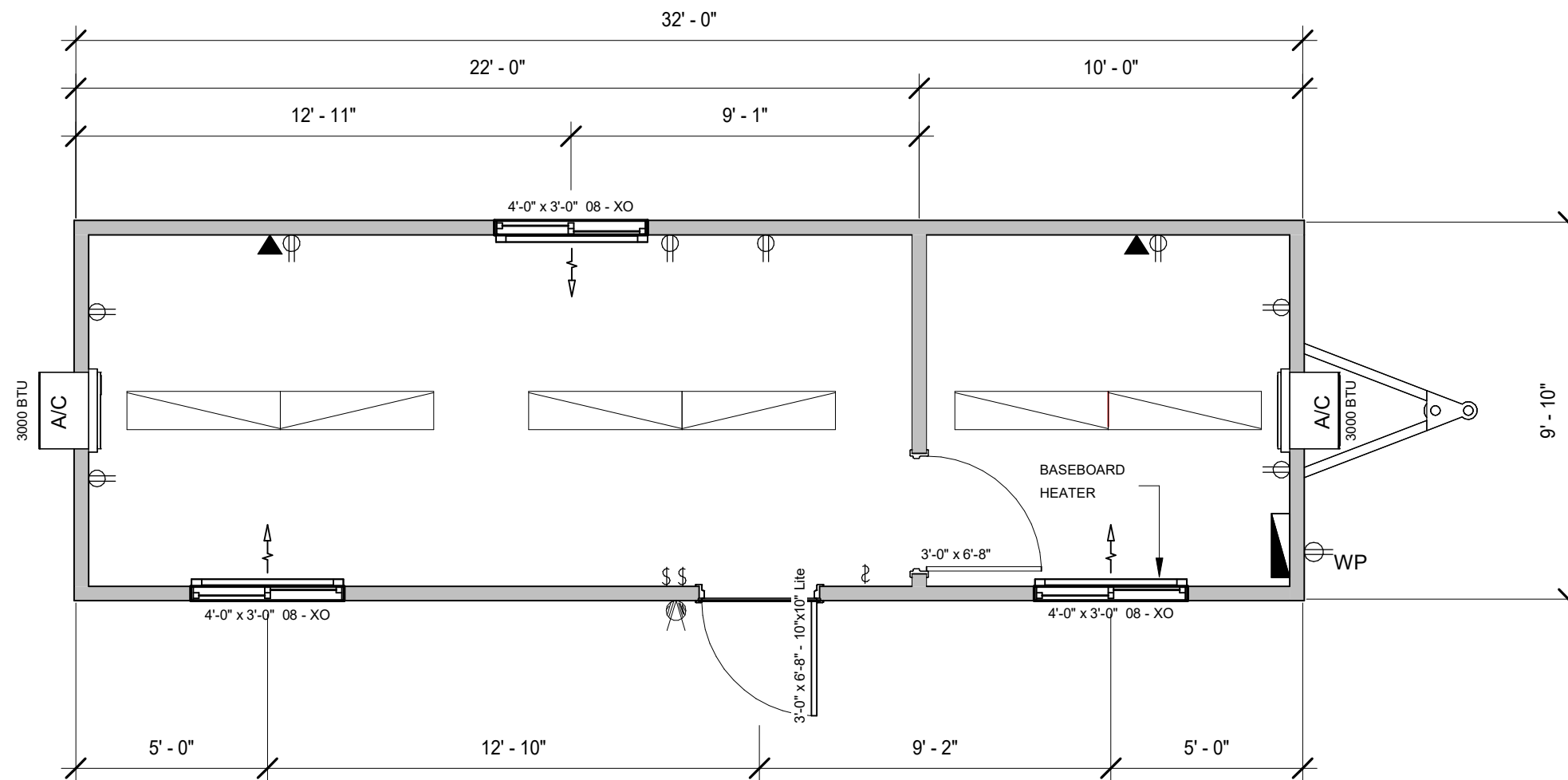
10' x 32' MOBILE OFFICE
