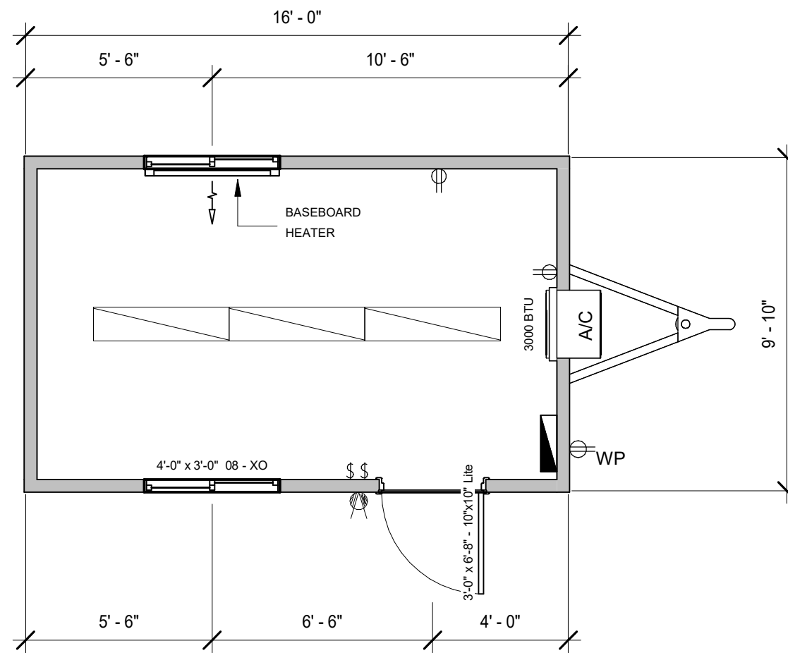
10' x 16' MOBILE OFFICE
