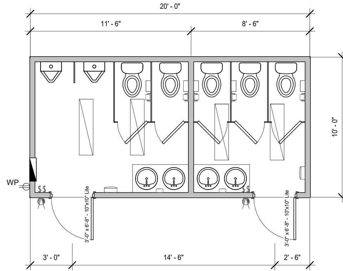
10' x 20' LAVATORY
