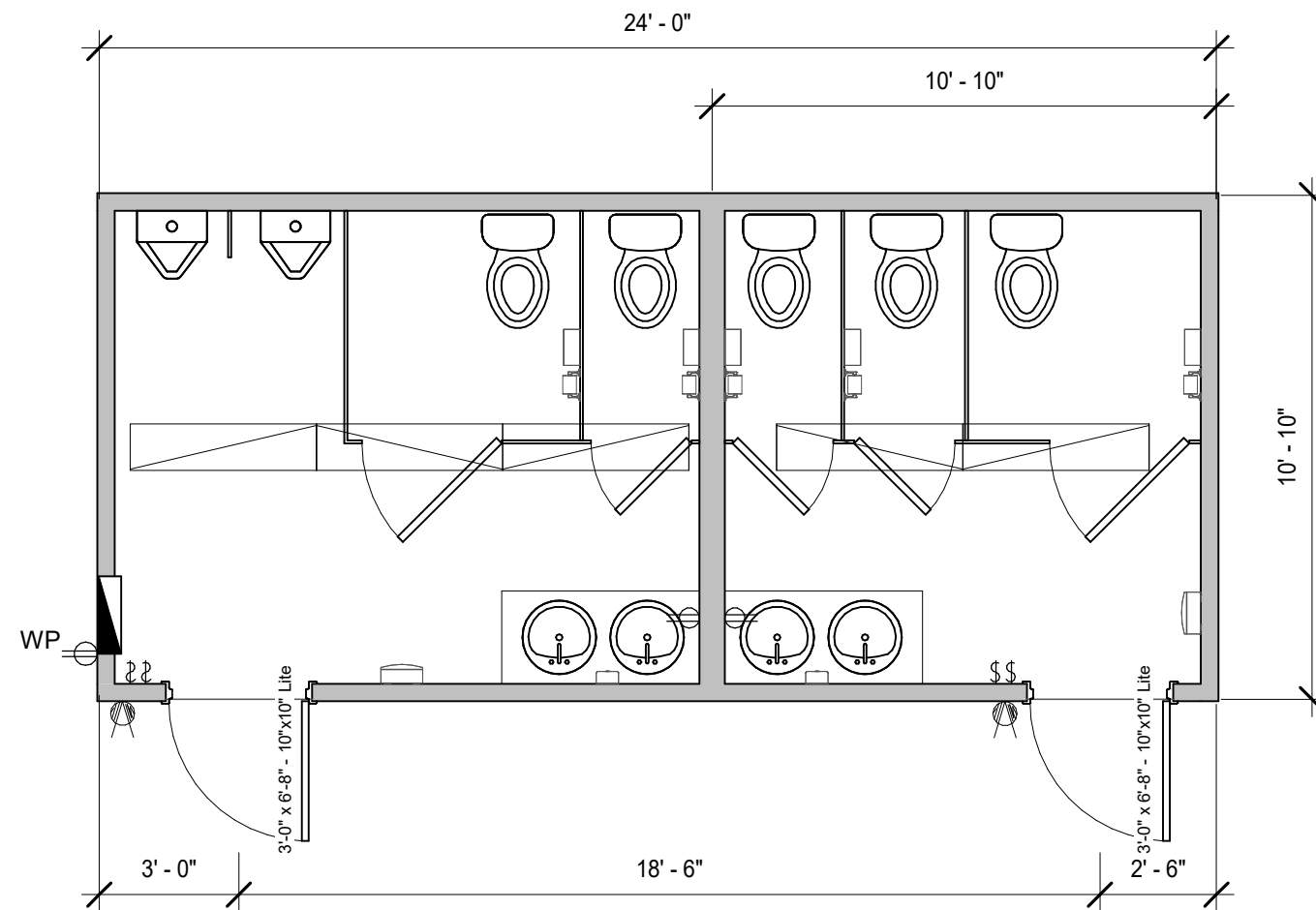
11' x 24' LAVATORY
