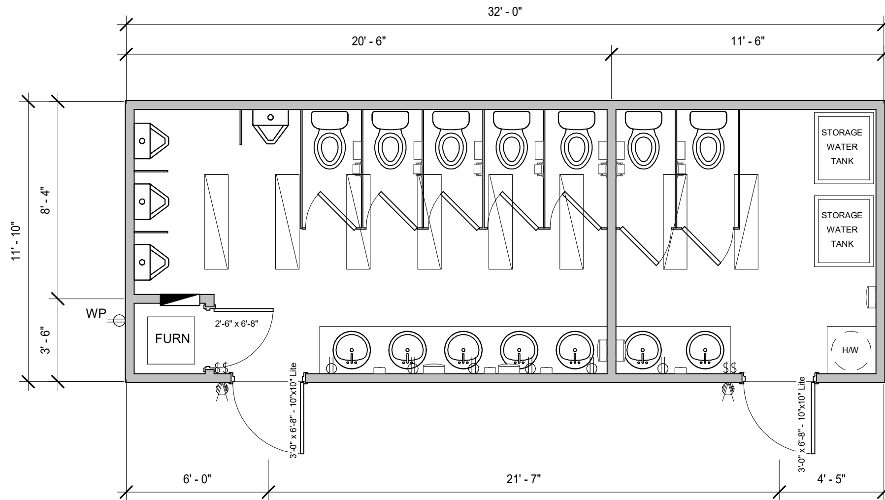
12' x 32' LAVATORY
