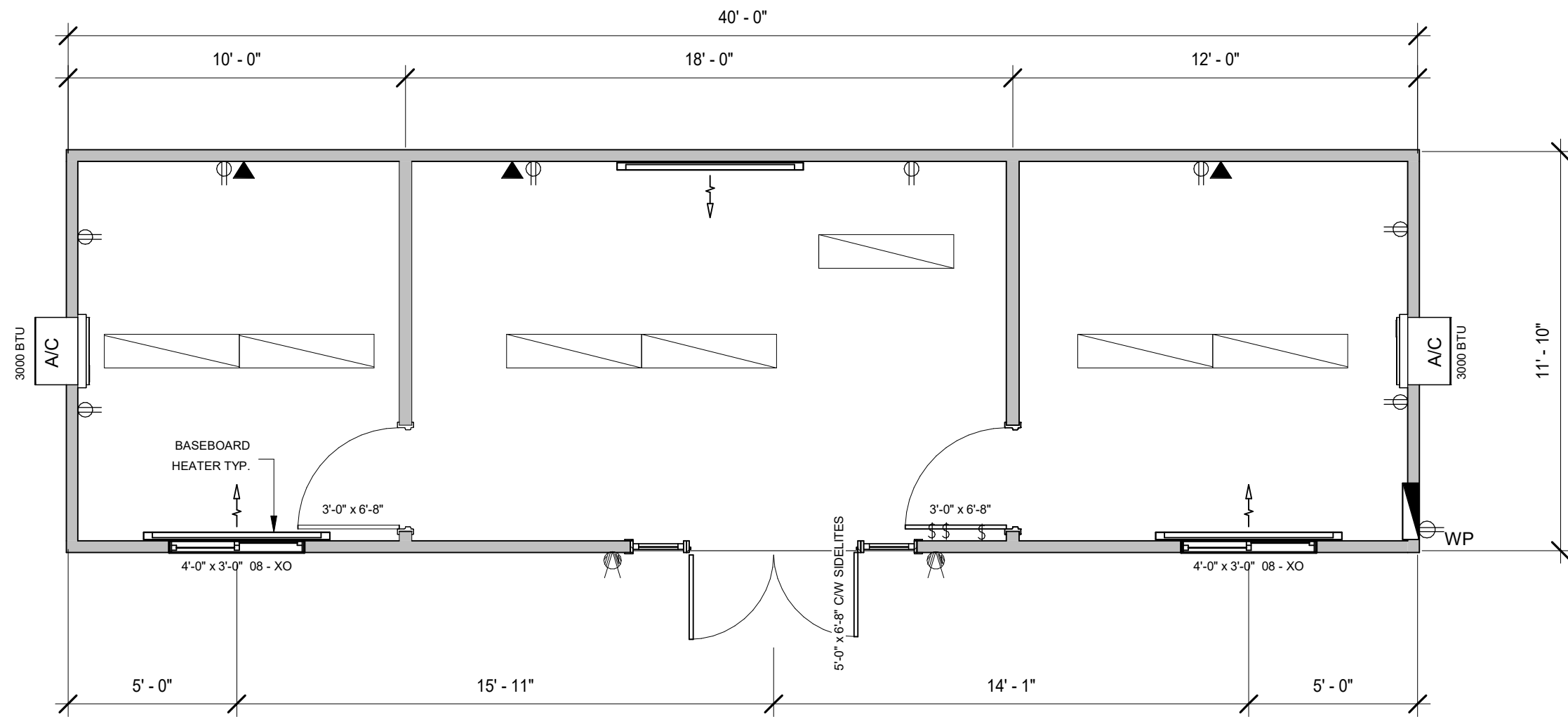
12' x 40' DESIGNER OFFICE
